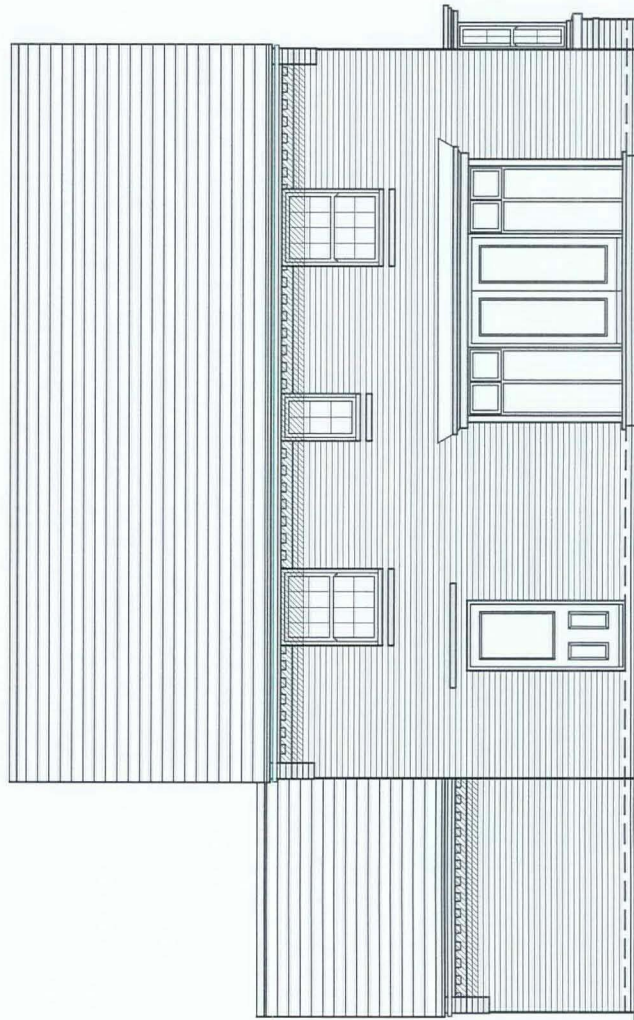
Rear Elevation
